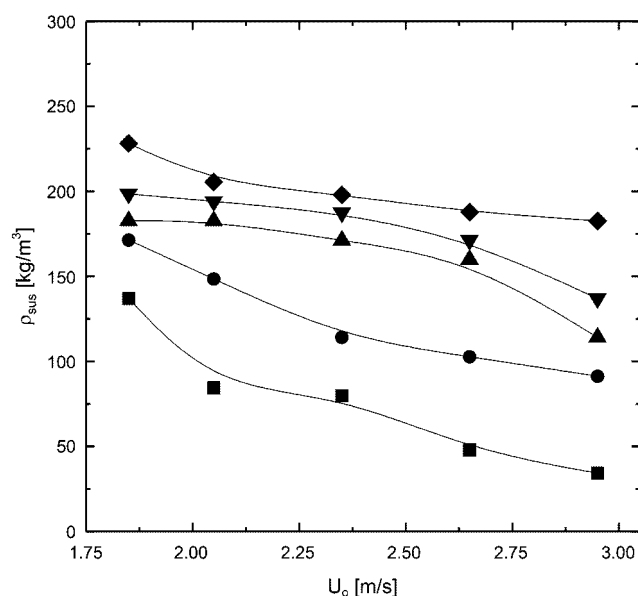
Fig. 10. Effects of gas velocity on the suspension density in the riser.
